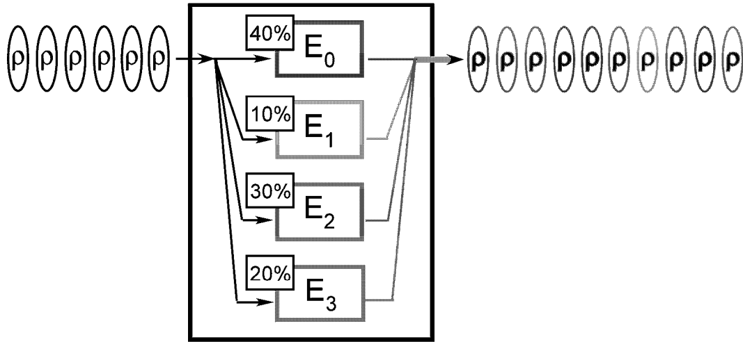
Fig. 6. An ensemble of single qubits are operated upon by an example of an arbitrary process. In general, any process can be represented by four orthogonal 2 \times 2 operators, each of which has some percentage chance of affecting an input qubit. These four operators have no restrictions, but they must in some way incoherently act upon input qubits. In this way input pure states affected by more than one operator can be transformed into a mixed ensemble.
